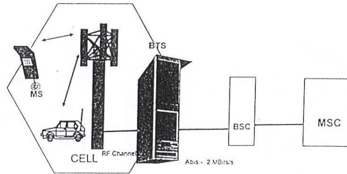
Figure 6: Cell Architecture:
