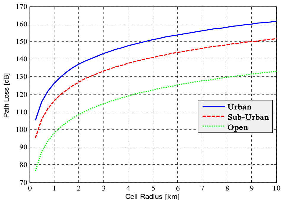
Figure 1: Path Loss as a Function of Cell Radius for Urban , Sub-Urban & Open Area .at f=900\text{MHz} , h(t)=30\text{m}
