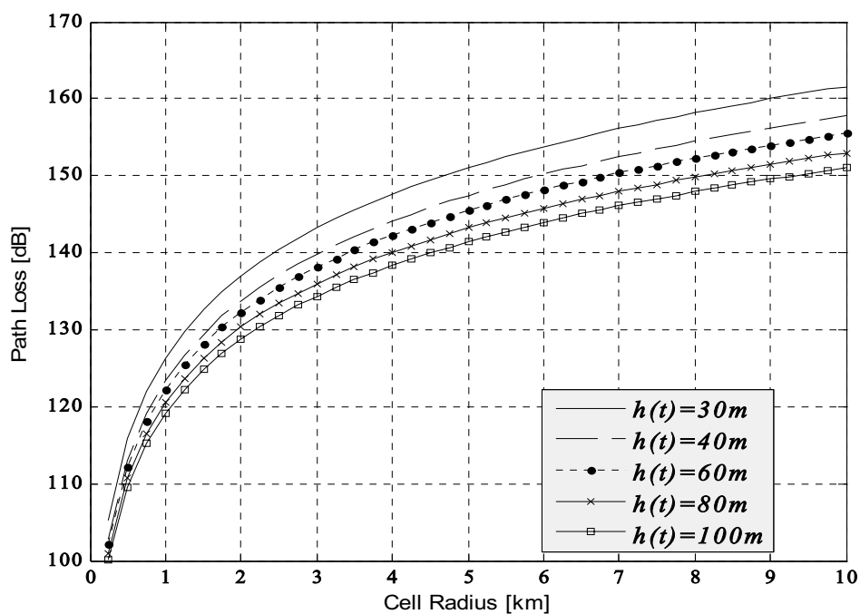
Figure 2: Path Loss versus Cell Radius for Urban Area at f = 900\text{MHz} , h(r) = 1.5\text{m}
