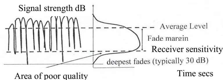
Figure 3: Small scale fading (Rayleigh fading) [9]
