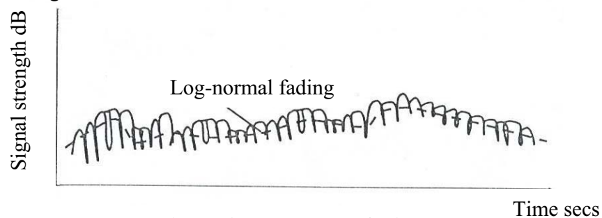
Figure 4: Log-normal fading
