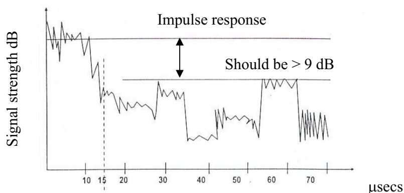
Figure 5: Time dispersion (Multipath). [10]
